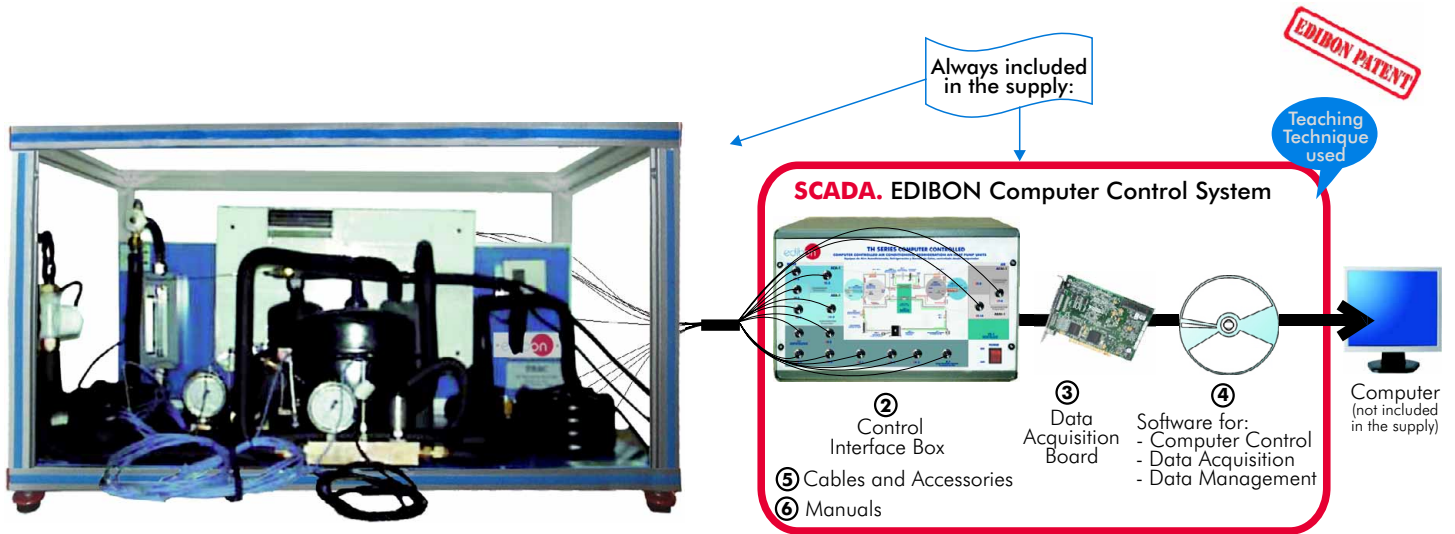
① Unit: THARL2C. Refrigeration and Air Conditioning Unit (one condenser (water) and two evaporators (water and air))
