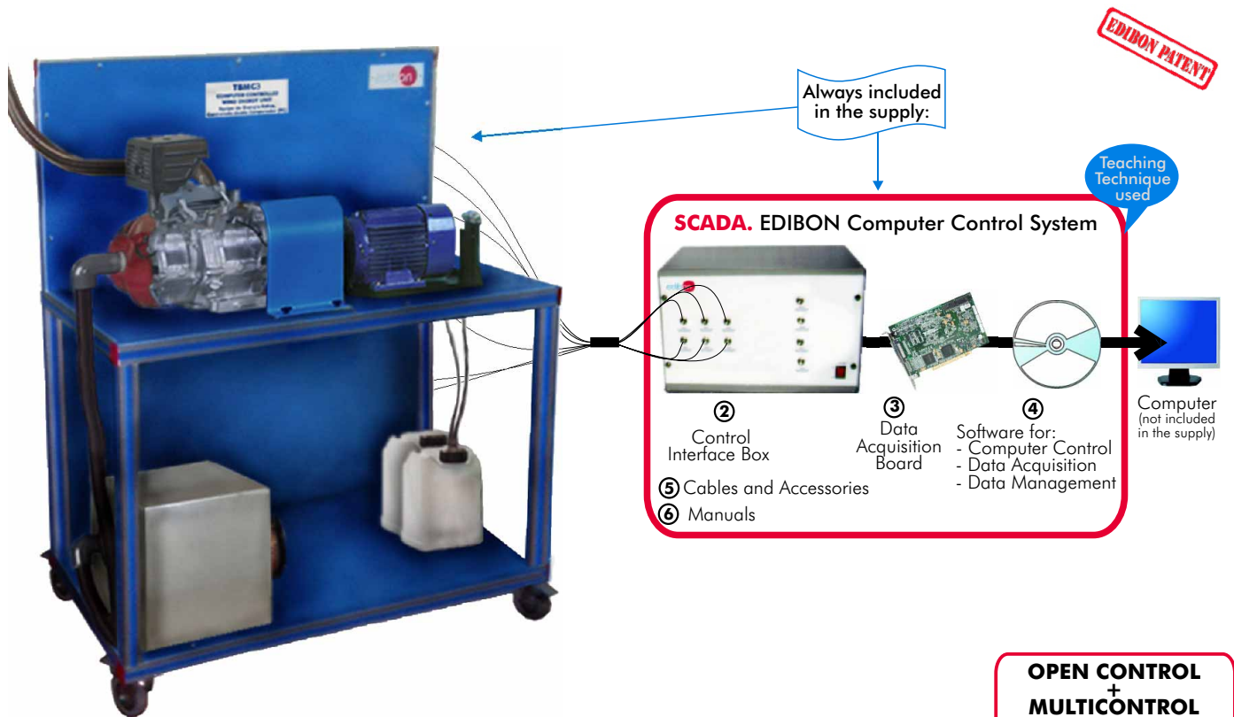
① Unit: TBMC3. Test Bench for Single-Cylinder Engines, 2.2 kW.
